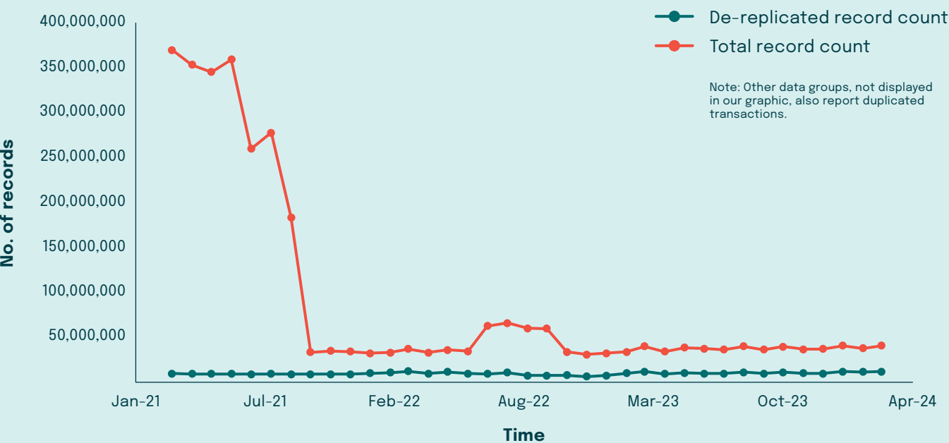
Graph 1 Effects of replication Total vs de-replicated record counts - by month
