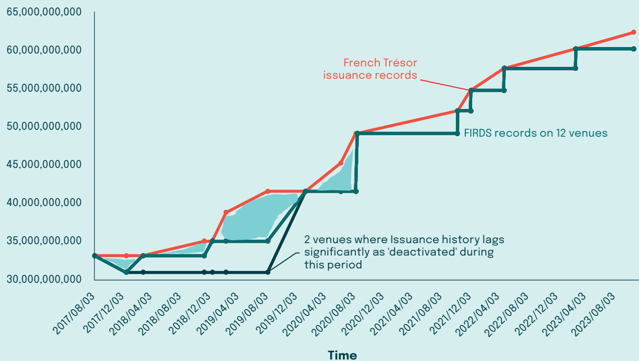
Graph 4 France 2.50% 30 May 2030 OAT issuance history
